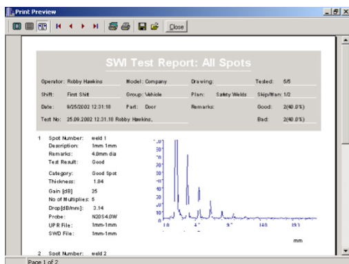
A-scan Report
